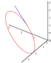
Figure 15.2.6 Path of the object with its initial velocity vector. (AP)
