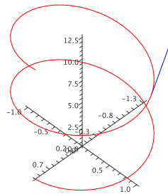
Figure 15.2.2 A tangent vector on the helix. (AP)
