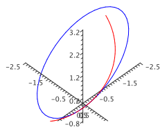
Figure 15.3.1 A circle with the same curvature as the helix. (AP)
