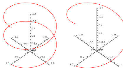
Figure 15.1.1 Two helices. (AP)
