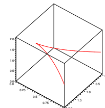
Figure 15.2.5 \langle 1 + t^3, t^2, 1 \rangle has a cusp at \langle 1, 0, 1 \rangle . (AP)
