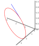
Figure 15.2.6 Path of the object with its initial velocity vector. (AP)
