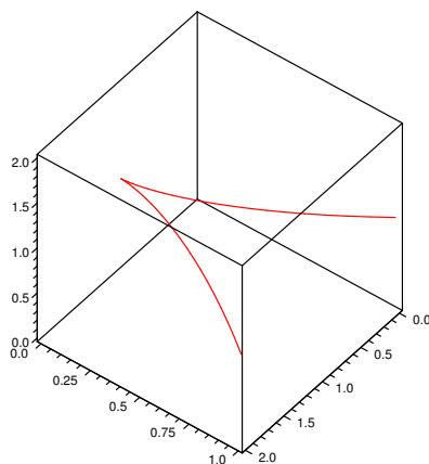
Figure 15.2.5 \langle 1 + t^3, t^2, 1 \rangle has a cusp at \langle 1, 0, 1 \rangle . (AP)
