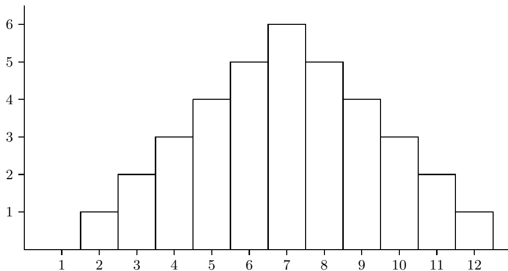
Figure 11.3.1 A probability density function for two dice.
