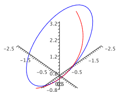
Figure 15.3.1 A circle with the same curvature as the helix.
