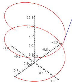
Figure 15.2.2 A tangent vector on the helix.
