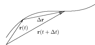
Figure 15.2.1 Approximating the derivative.
