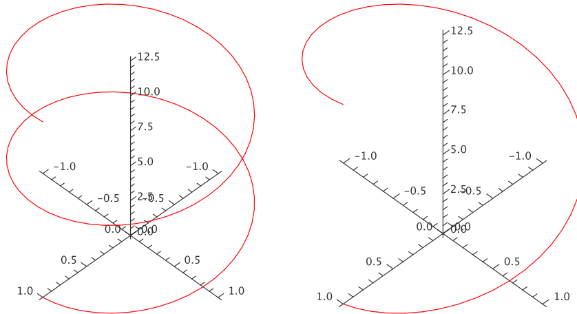
Figure 15.1.1 Two helices.
