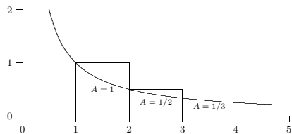
Figure 13.3.2 Graph of y = 1/x with rectangles.
