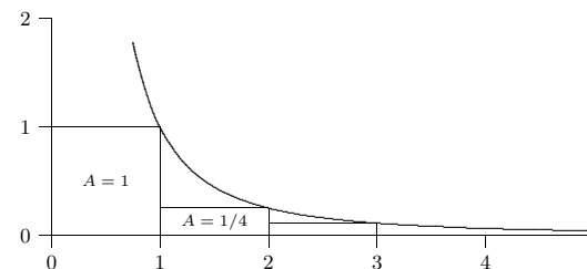
Figure 13.3.1 Graph of y = 1/x^2 with rectangles.
