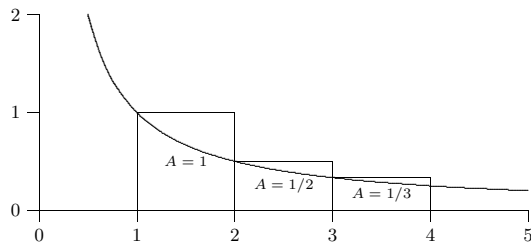
Figure 13.3.2 Graph of y = 1/x with rectangles.
