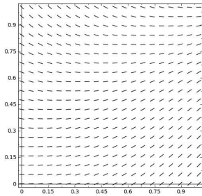
Figure 19.2 A slope field for \dot{y} = t - y^2 .
