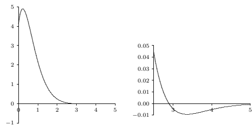
Figure 19.4 Graph of a damped oscillation.
