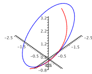
Figure 15.9 A circle with the same curvature as the helix. (AP)
