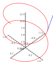
Figure 15.4 A tangent vector on the helix. (AP)
