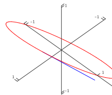
Figure 15.5 The ellipse \mathbf{r} = \langle \cos t, \sin t, \cos t \rangle . (AP)
