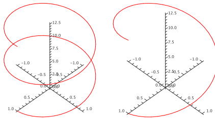
Figure 15.1 Two helices. (AP)
