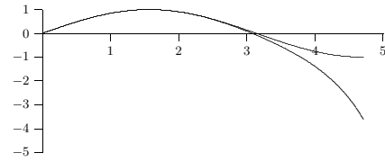
Figure 13.5 \sin x and a polynomial approximation. (AP)
