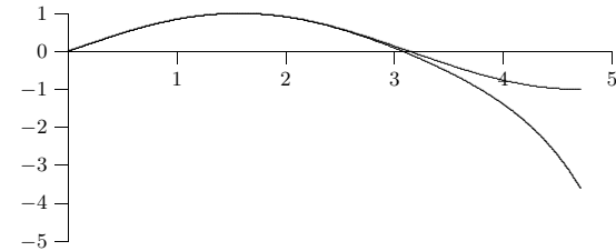
Figure 13.5 \sin x and a polynomial approximation. (AP)
