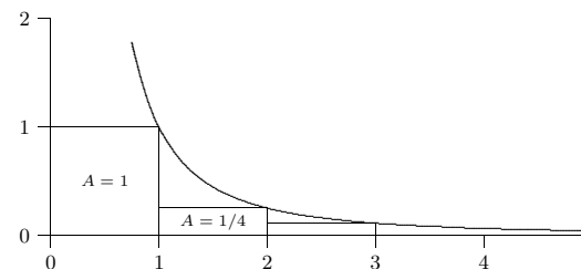
Figure 13.2 Graph of y = 1/x^2 with rectangles.
