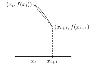
Figure 10.2 A single trapezoid.
