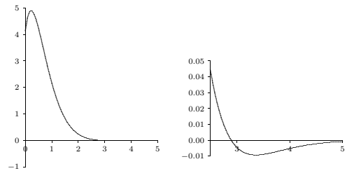
Figure 19.4 Graph of a damped oscillation.
