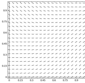
Figure 19.2 A slope field for \dot{y} = t - y^2 .
