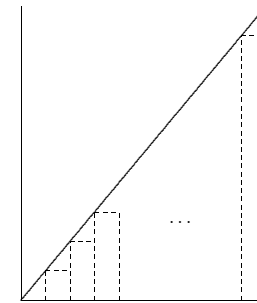
Figure 7.1 Approximating the area under y = 3x with rectangles.
