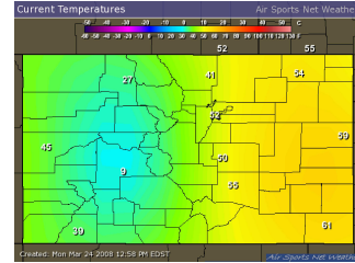
Figure 15.1.5 Colorado temperatures.
