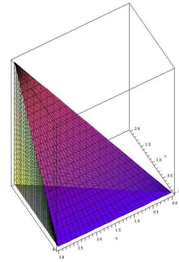
Figure 15.5.1 A tetrahedron.
