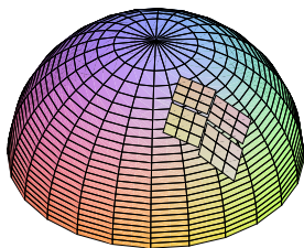
Figure 15.4.1 Small parallelograms at points of tangency.
