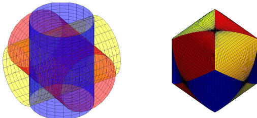
Figure 15.1.6 Intersection of three cylinders.
