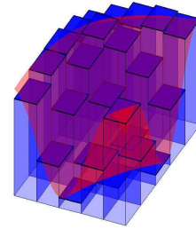
Figure 15.1.2 Approximating the volume under a surface.
