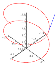
Figure 13.2.2 A tangent vector on the helix.
