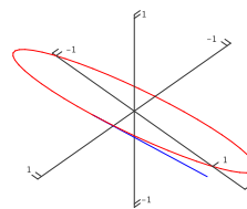
Figure 13.2.3 The ellipse \mathbf{r} = \langle \cos t, \sin t, \cos t \rangle .
