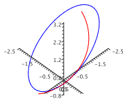
Figure 13.3.1 A circle with the same curvature as the helix.
