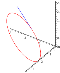
Figure 13.2.6 Path of the object with its initial velocity vector.
