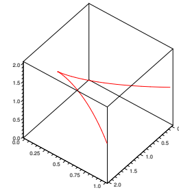
Figure 13.2.5 \langle 1 + t^3, t^2, 1 \rangle has a cusp at (1, 0, 1) .
