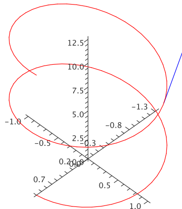
Figure 13.2.2 A tangent vector on the helix.
