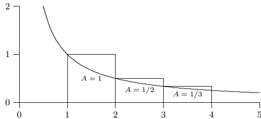
Figure 11.3.2 Graph of y = 1/x with rectangles.
