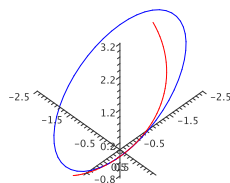
Figure 13.9 A circle with the same curvature as the helix. (AP)
