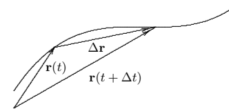
Figure 13.3 Approximating the derivative.
