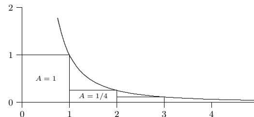
Figure 11.2 Graph of y = 1/x^2 with rectangles.
