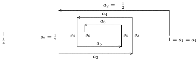
Figure 11.4 The alternating harmonic series.
