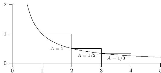
Figure 11.3 Graph of y = 1/x with rectangles.
