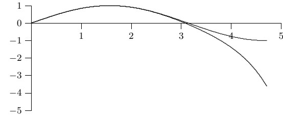
Figure 11.5 \sin x and a polynomial approximation. (AP)
