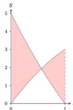
Figure 9.1.4 Area between curves that cross.
