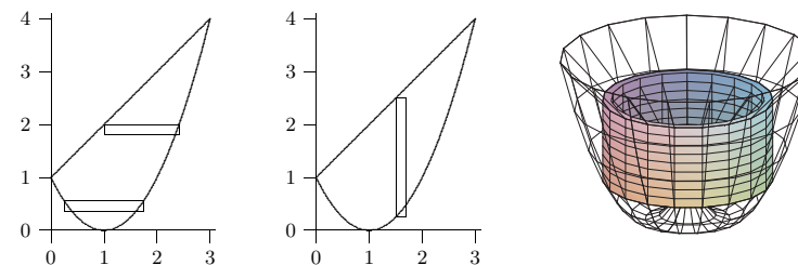
Figure 9.3.6 Computing volumes with “shells”. (AP)
