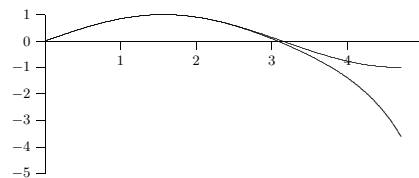
Figure 13.5 \sin x and a polynomial approximation.
