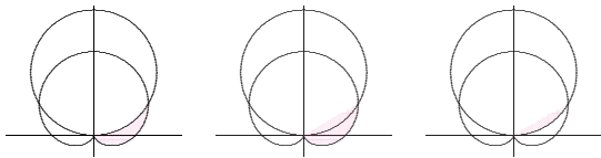
Figure 12.9 An area between curves.
