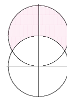
Figure 12.8 An area between curves.
