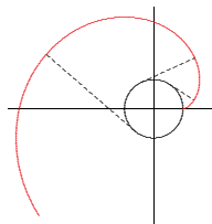
Figure 12.14 An involute of a circle.
