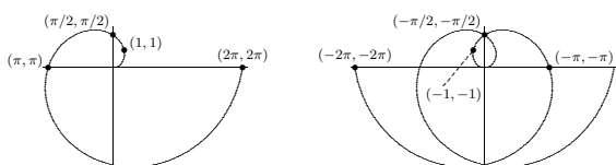
Figure 12.4 The spiral of Archimedes and the full graph of r = \theta .
