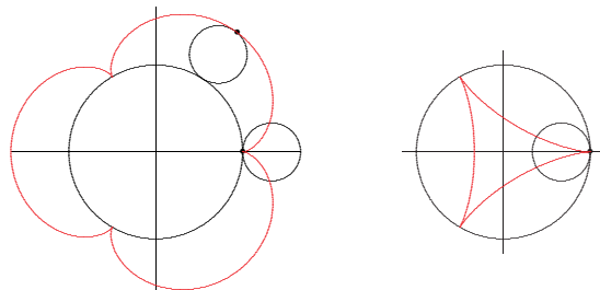
Figure 12.13 A hypercycloid and a hypocycloid.
