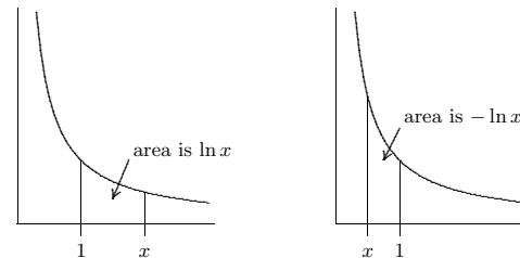
Figure 9.1 \ln(x) is an area.
