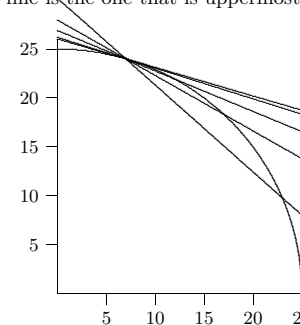
Figure 2.1 Chords approximating the tangent line.
