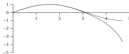
Figure 13.11.1 \sin x and a polynomial approximation. (AP)
