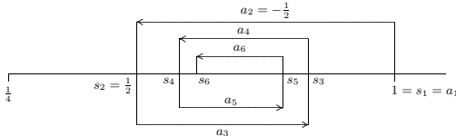
Figure 13.4.1 The alternating harmonic series.
