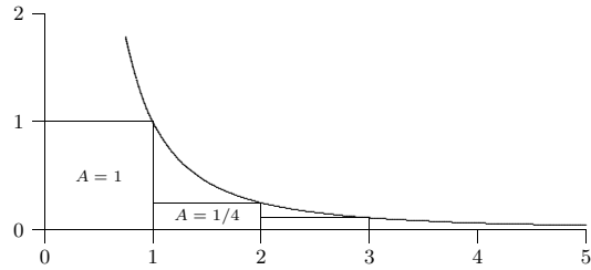
Figure 11.3.1 Graph of y = 1/x^2 with rectangles.
