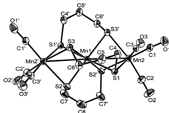
Figure 3. Molecular structure of \text{Mn}_3(\text{CO})_6(\mu\text{-}\eta^4\text{-SCH}_2\text{CH}_2\text{CH}_2\text{S})_3 ( 6 ) showing the atom-labeling scheme; thermal ellipsoids are drawn at the 50% probability level.
