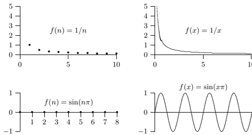
Figure 13.1 Graphs of sequences and their corresponding real functions.
