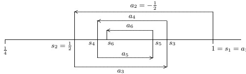
Figure 13.4 The alternating harmonic series.
