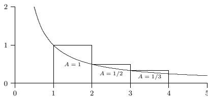
Figure 13.3 Graph of y = 1/x with rectangles.
