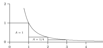
Figure 13.2 Graph of y = 1/x^2 with rectangles.
