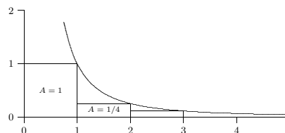
Figure 11.2 Graph of y = 1/x^2 with rectangles.
