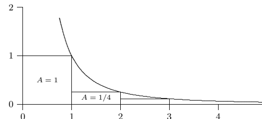
Figure 11.2 Graph of y = 1/x^2 with rectangles.
