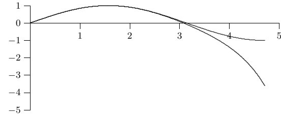
Figure 11.5 \sin x and a polynomial approximation. (AP)
