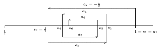
Figure 10.4 The alternating harmonic series.
