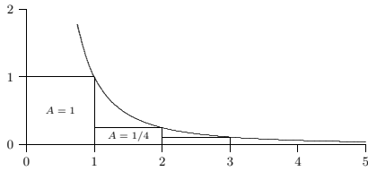
Figure 10.2 Graph of y = 1/x^2 with rectangles.
