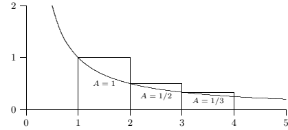
Figure 10.3 Graph of y = 1/x with rectangles.
