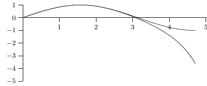
Figure 10.5 \sin x and a polynomial approximation.
